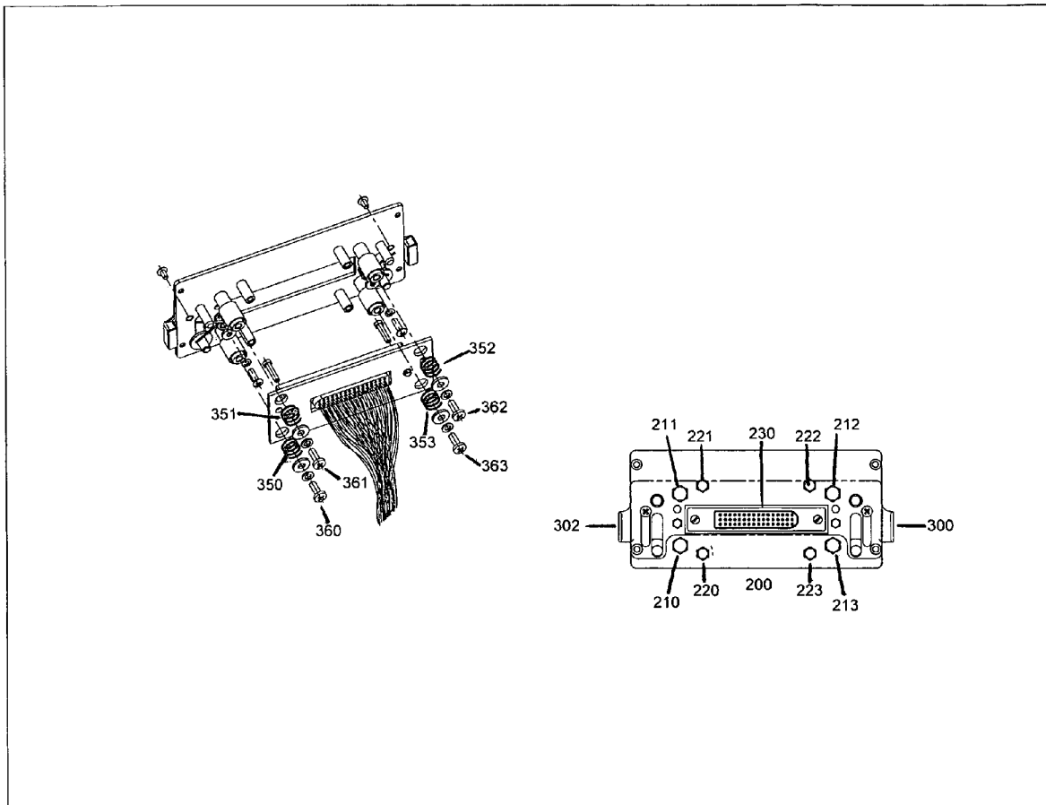
Assembly view with stop posts, springs, and spring posts
